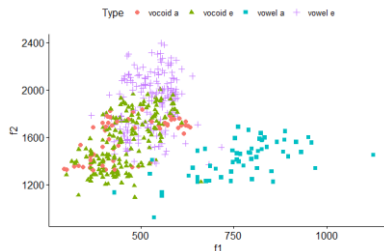
Figure 4: f1 and f2 values for /a/, /e/, and vocoids preceding either /a/ or /e/.
